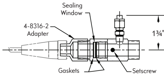
8831-R 4 1/2" long Shown with UV-2 UV Scanner
