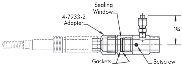
8836-R 4 1/2" long Shown with UV7A4 UV Scanner
