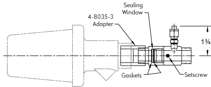
8839-R 4 1/2" long Shown with 45UV5 UV Scanner
