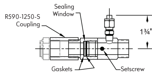
8834-R 5" long Shown with 8790-0 Observation Port
