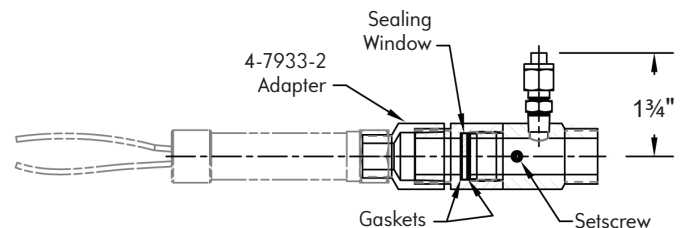
8836-R 4 1/2" long Shown with C7027A UV Scanner
