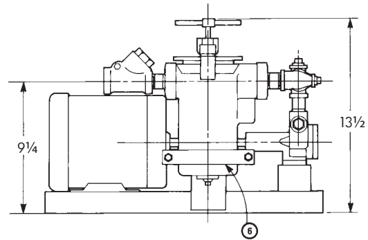
8563- -A Packaged Pump Set for Light Oil
