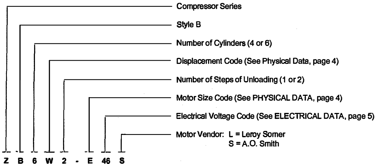
FIG. 1 — COMPRESSOR DATA PLATE
