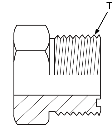
FIGURE 12 - ORFS TUBE END PLUG
