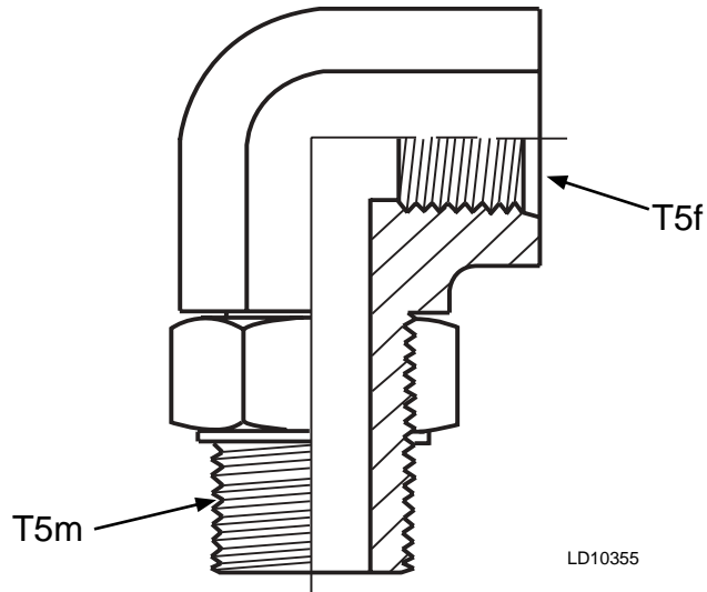
FIGURE 22 - STRAIGHT THREAD ELBOW
