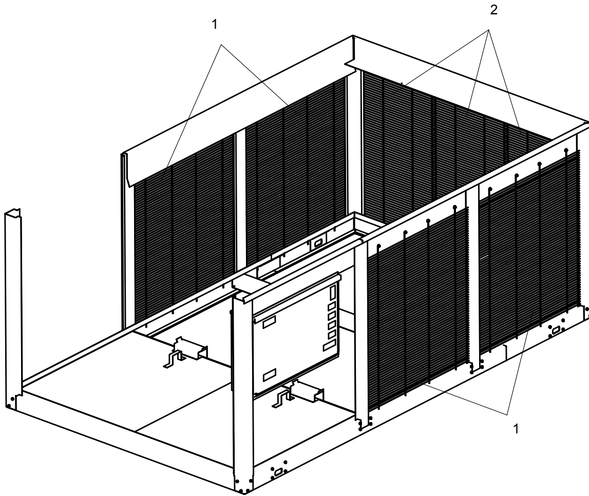
FIGURE 21 - WIRE ENCLOSURE PARTS
