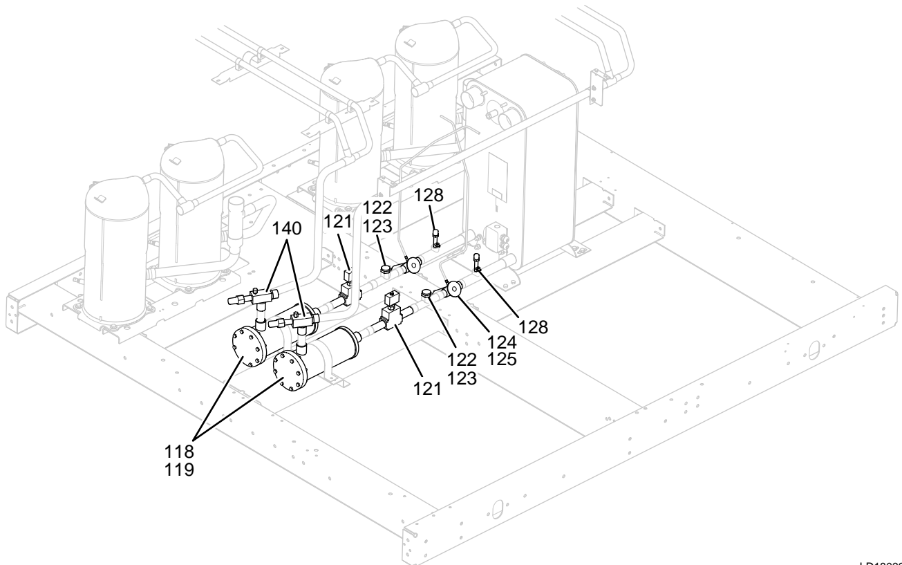
FIGURE 7 - SYSTEM PIPING (QTC3055T, QTC3060T, QTC3080T)
