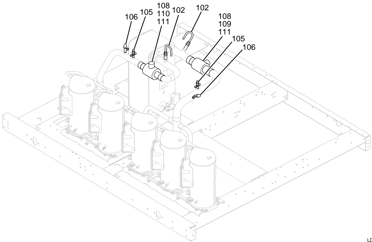
FIGURE 6 - SYSTEM PIPING (QTC3055T, QTC3060T, QTC3080T)
